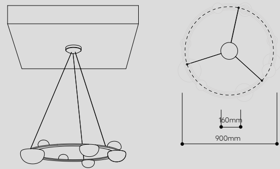
Dew Drops Circle – Centered canopy for solid ceiling (power source in the canopy)
